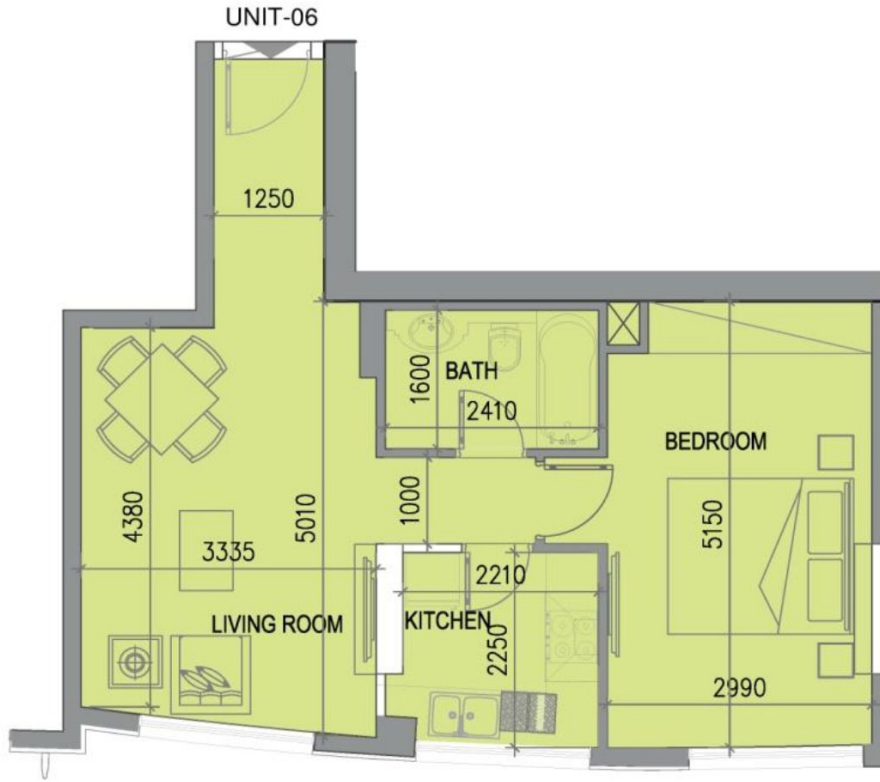
UNIT-6 (1B) AREA - 490.19 SQFT
